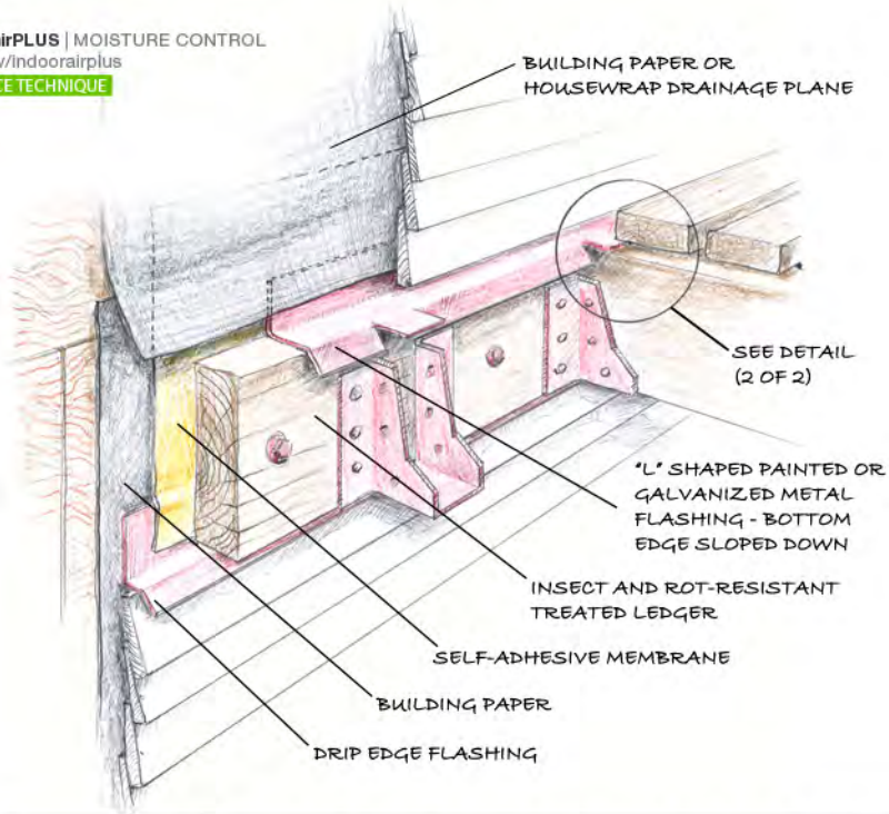
FLASHING DIVERTING WATER FROM DECK LEDGER (1 OF 2)
