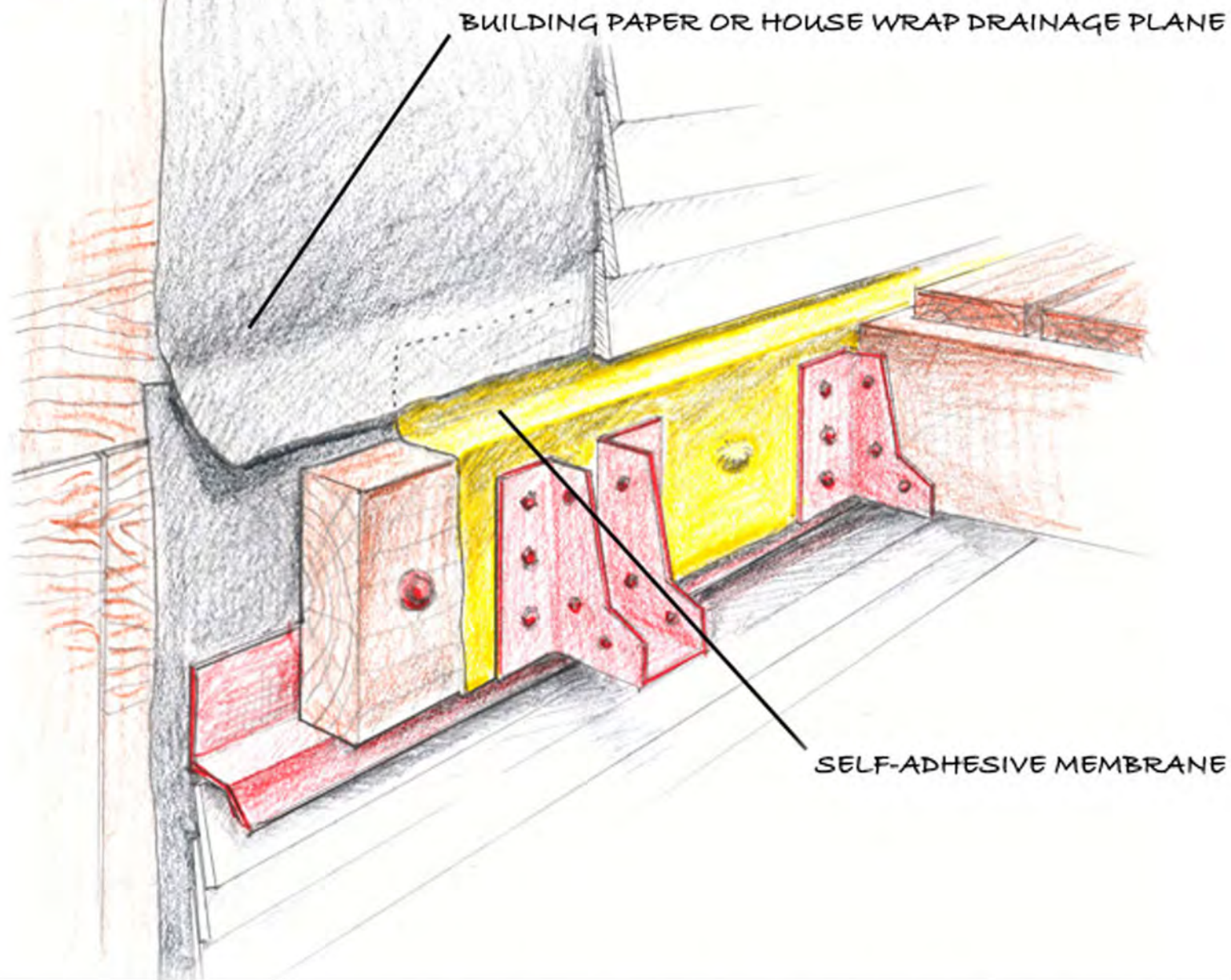
FLASHING A LEDGER BOARD WITH MEMBRANE MATERIAL
